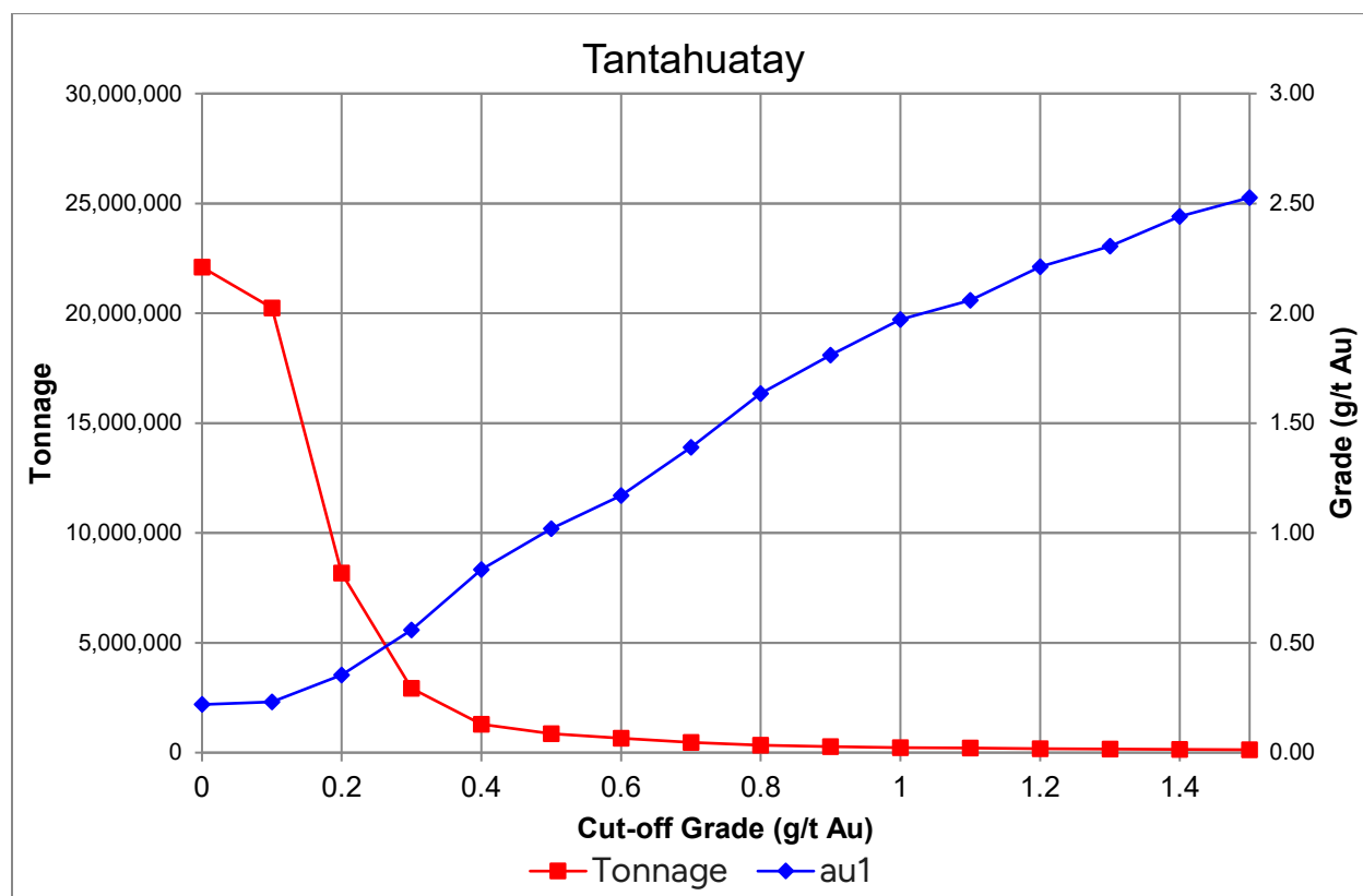
Figure 11-16: Grade-Tonnage Curve: Tantahuatay
