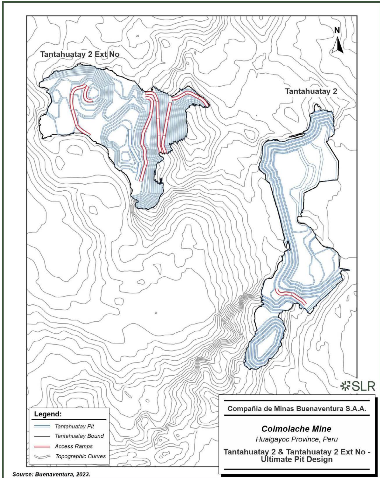
Figure 13-8: Tantauatay 2 and Tantauatay 2 Ext No Ultimate Pit Design
