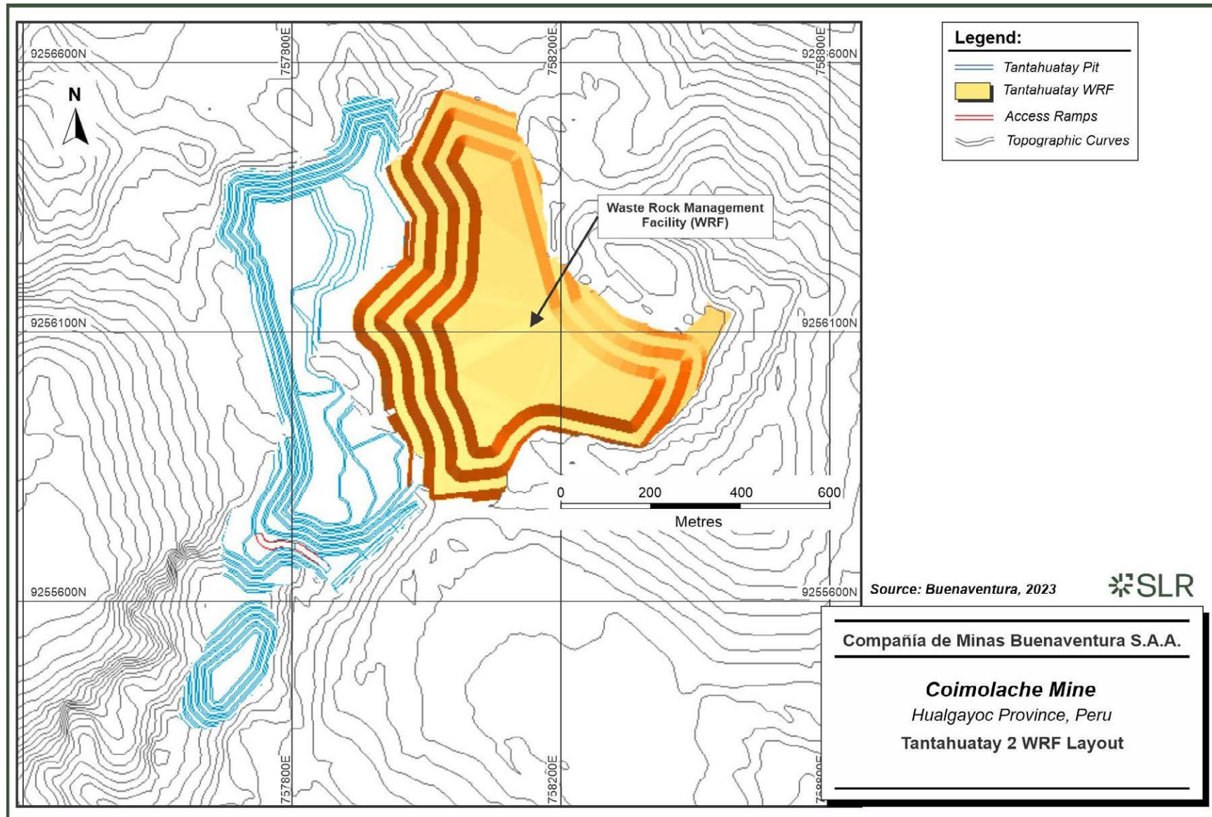
Figure 15-2: Tantauatay 2 WRF Layout
