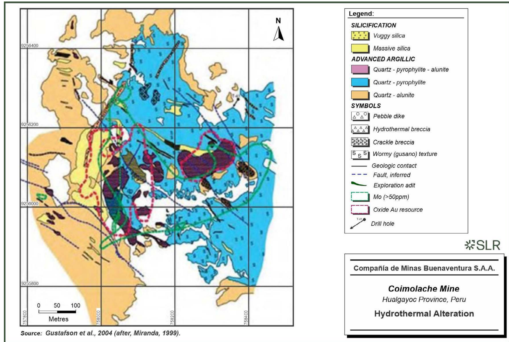
Figure 6-5: Hydrothermal Alteration
