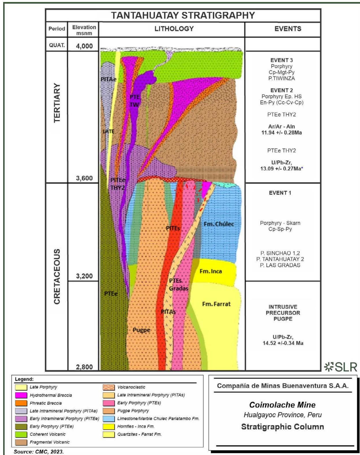
Figure 6-4: Stratigraphic Column
