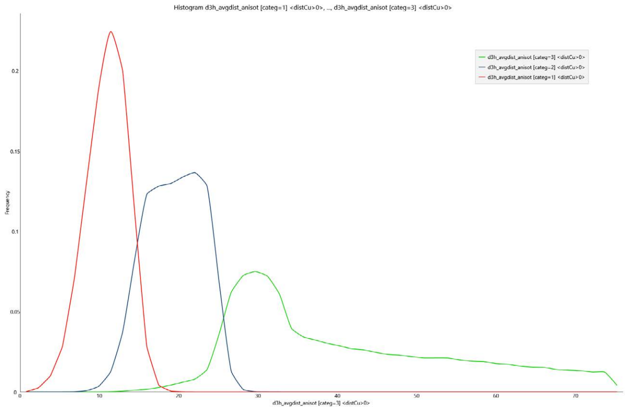
Figure 11-24: Classification Distances
