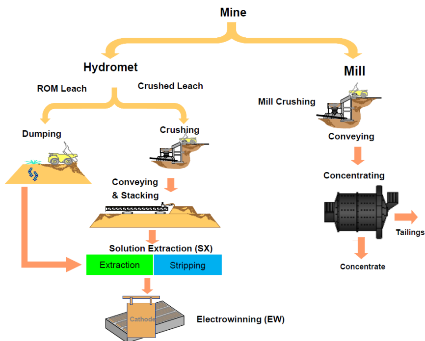
Figure 14.1 – Site Process Diagram
