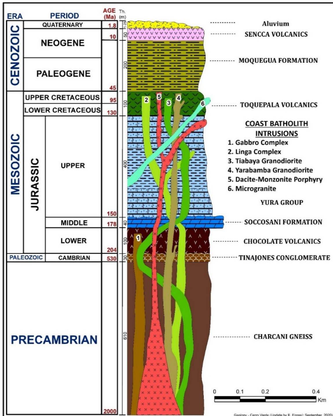
Figure 6.2 – Regional Stratigraphic Column of the CV and SR Deposits
