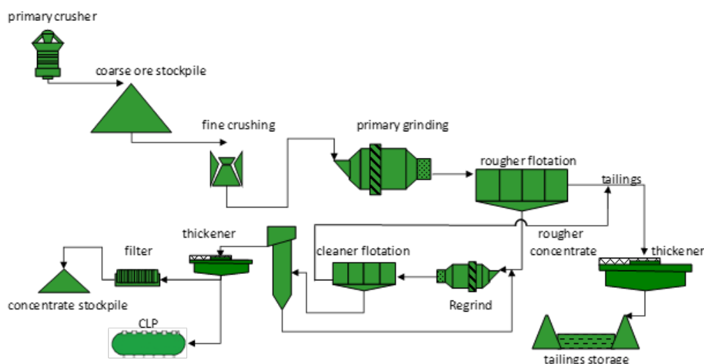
Figure 14.4 – Morenci and Metcalf Concentrator Process Flow Diagram
