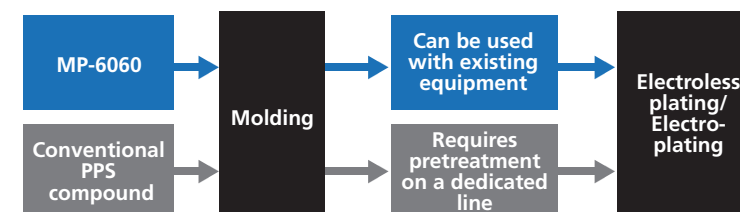
Process for plating newly developed PPS compound
