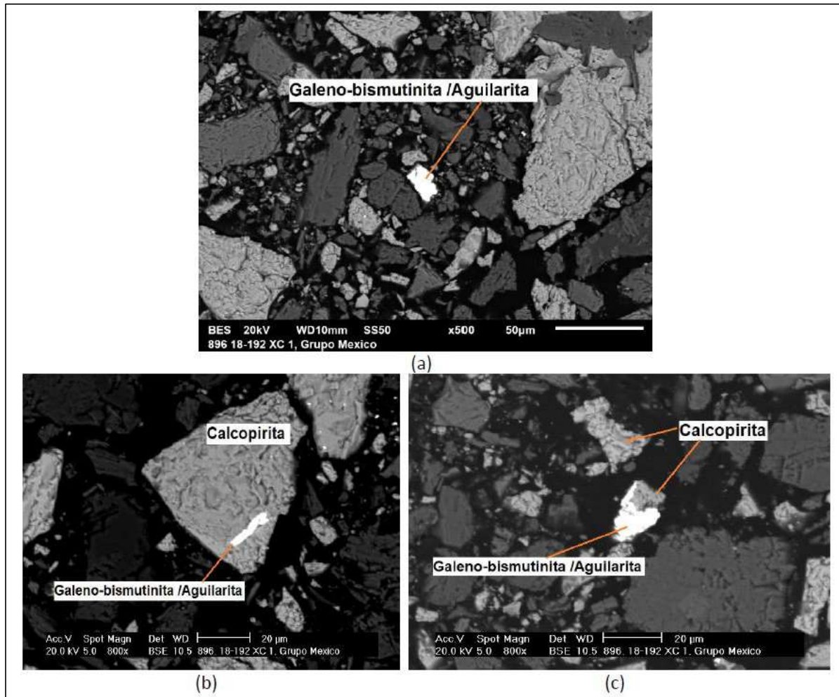
Figure 6-6: Galena-Bismuthinite/Aguilarite
