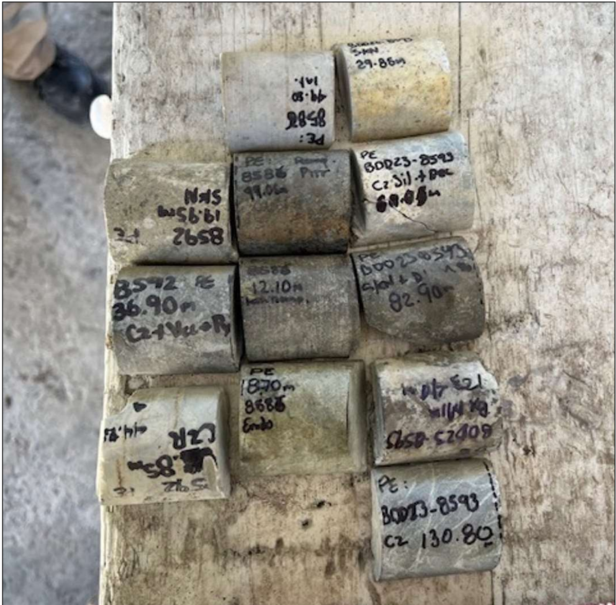
Figure 8-2: Core Samples for Density Testing
