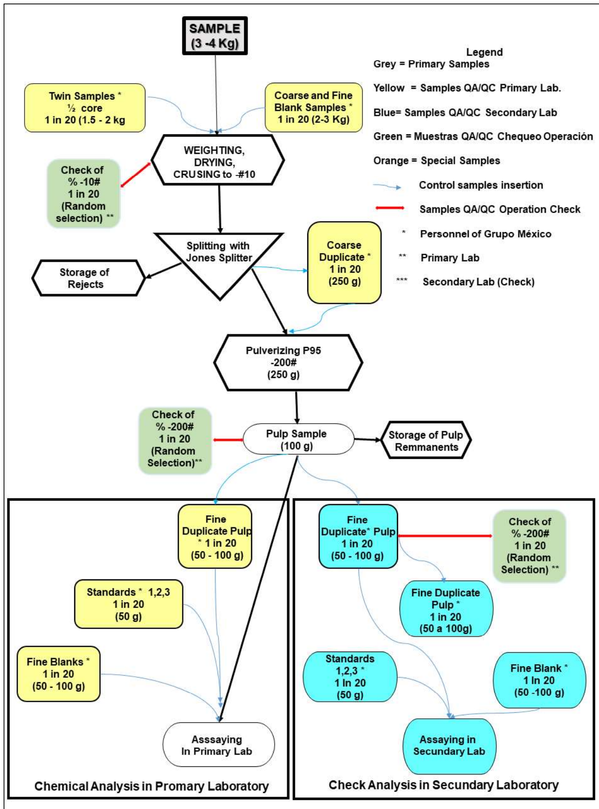
Figure 8-3: Flow Chart of Sample Preparation (Internal Laboratory)
