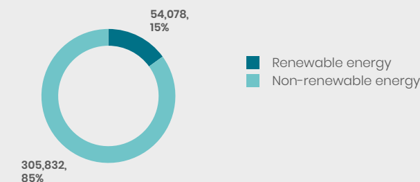
Energy mix (in MWh)
